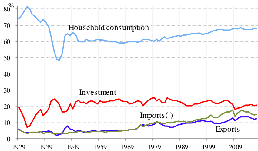
Appendix Figure 8: Historical Final Demand Shares of the US since 1929 —Share of final demands with respect to GDP at current market prices in 1929–2017 Sources: National Income and Production Accounts (NIPA), Bureau of Economic Analysis, US.
